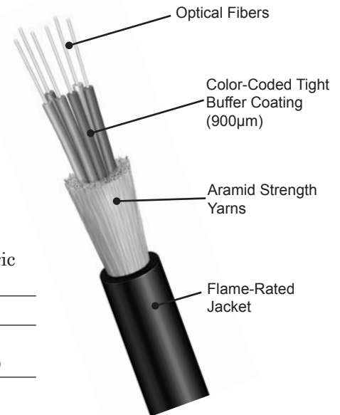
6-Fiber Cable
